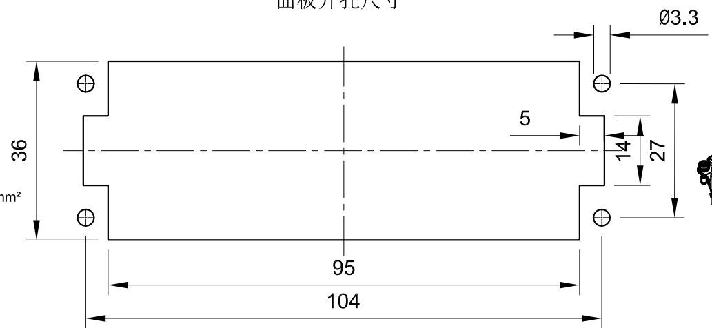
Panel cut out 面板开孔尺寸
